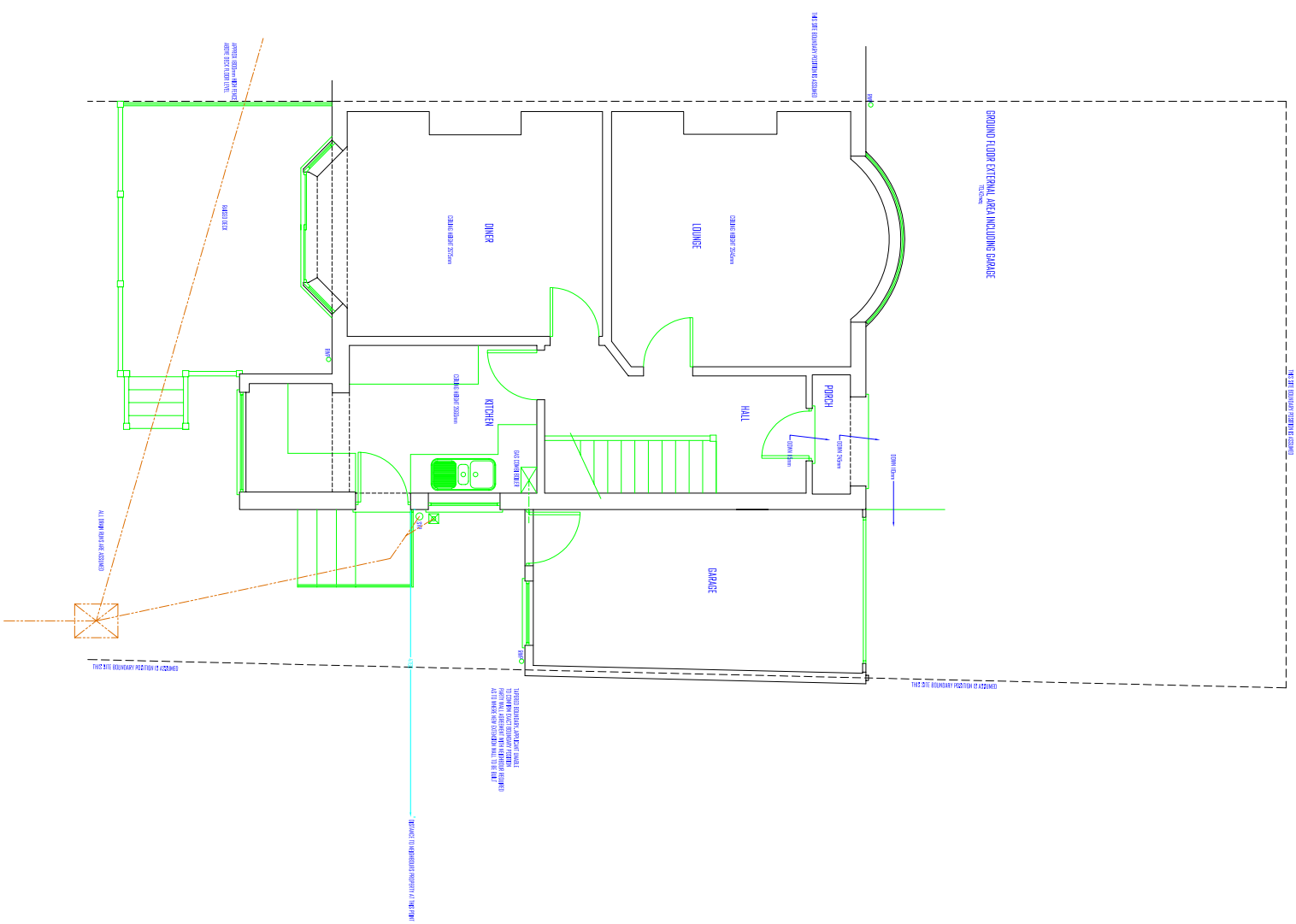
EXISTING GROUND FLOOR PLAN (1:100) @ A3
