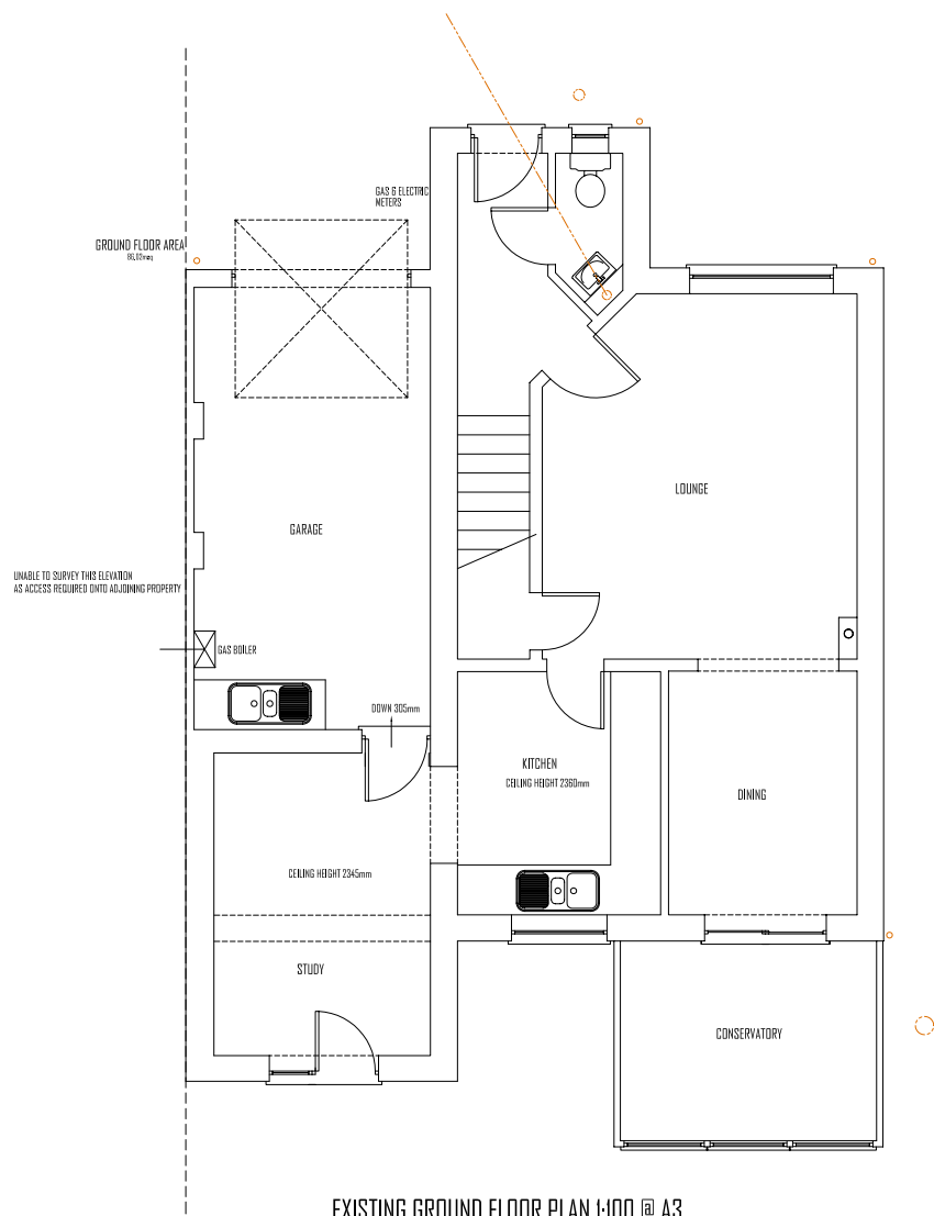
EXISTING GROUND FLOOR PLAN 1:100 @ A3
